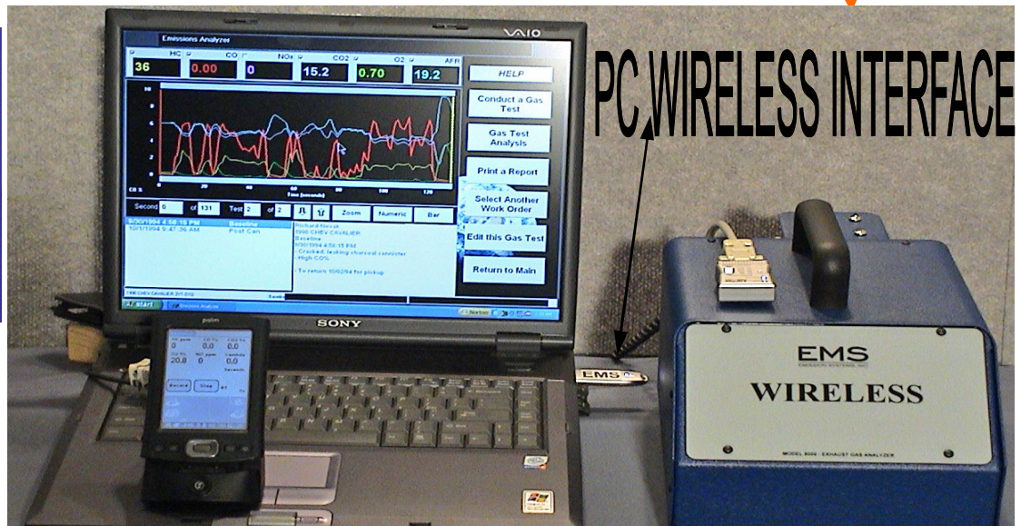
WIRELESS ANALYZER WITH BLUE TOOTH PALM PILOT OR WITH WIRELESS PC INTERFACE
